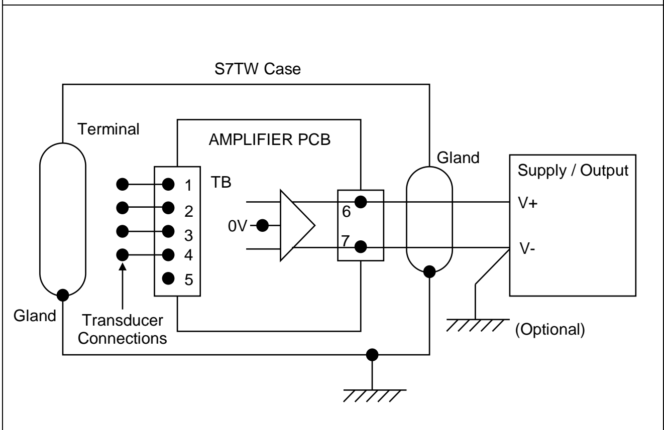
Fig. 3 Connection Schematic
